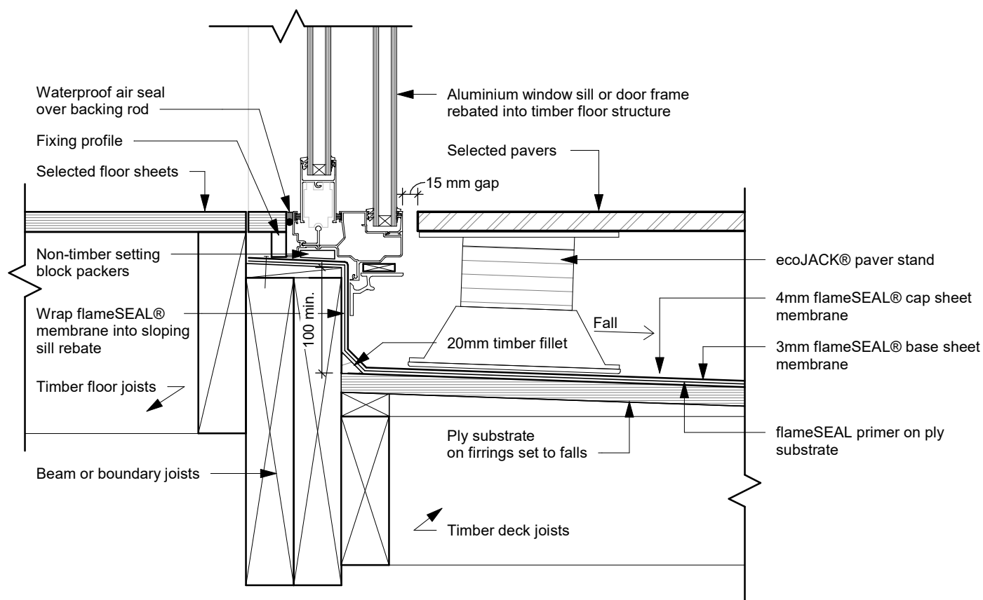
fS D33 - ecoJACK® Paver - Threshold Detail - Type 1
