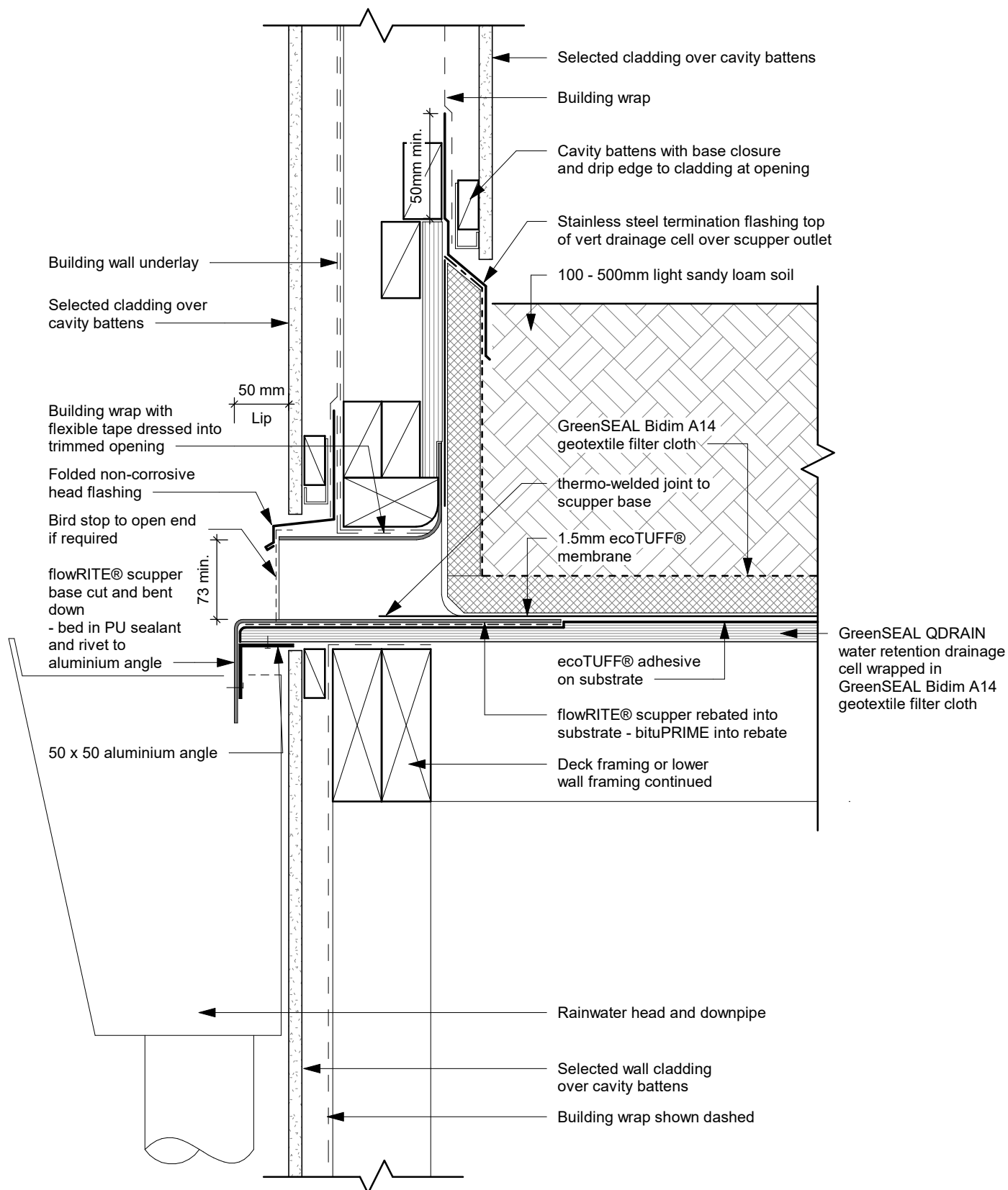
eT D08 - (TPO) Soil flowRITE® Scupper
