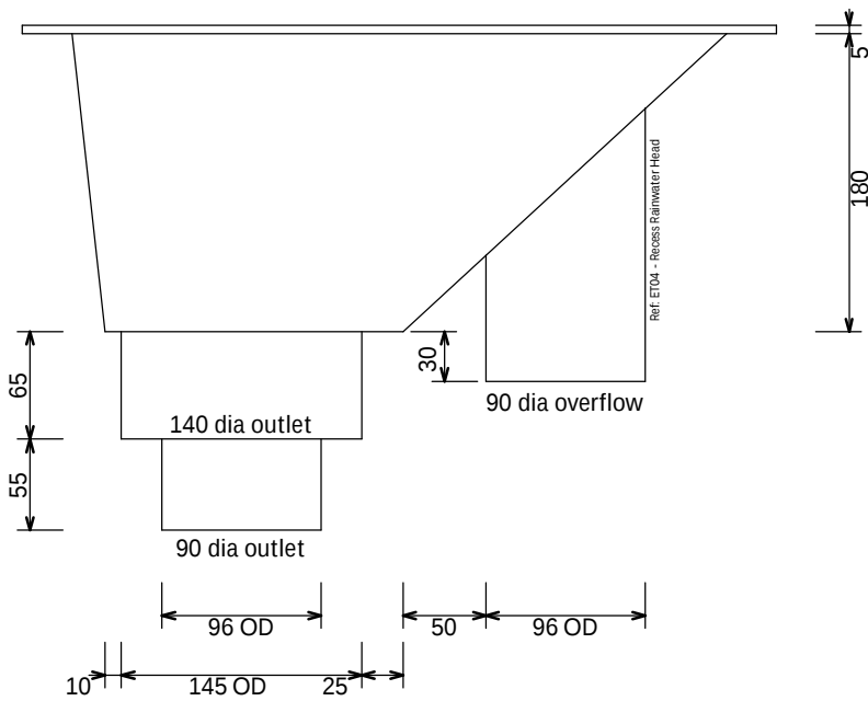
Recessed Internal Gutter Rainwater Head
