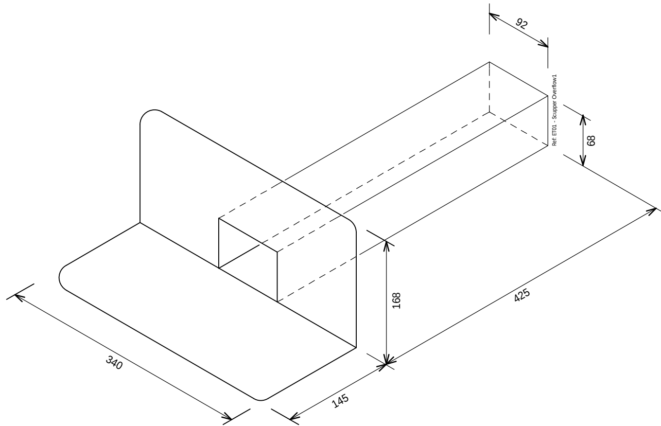
Eterno™ Scupper Overflow 65mm
