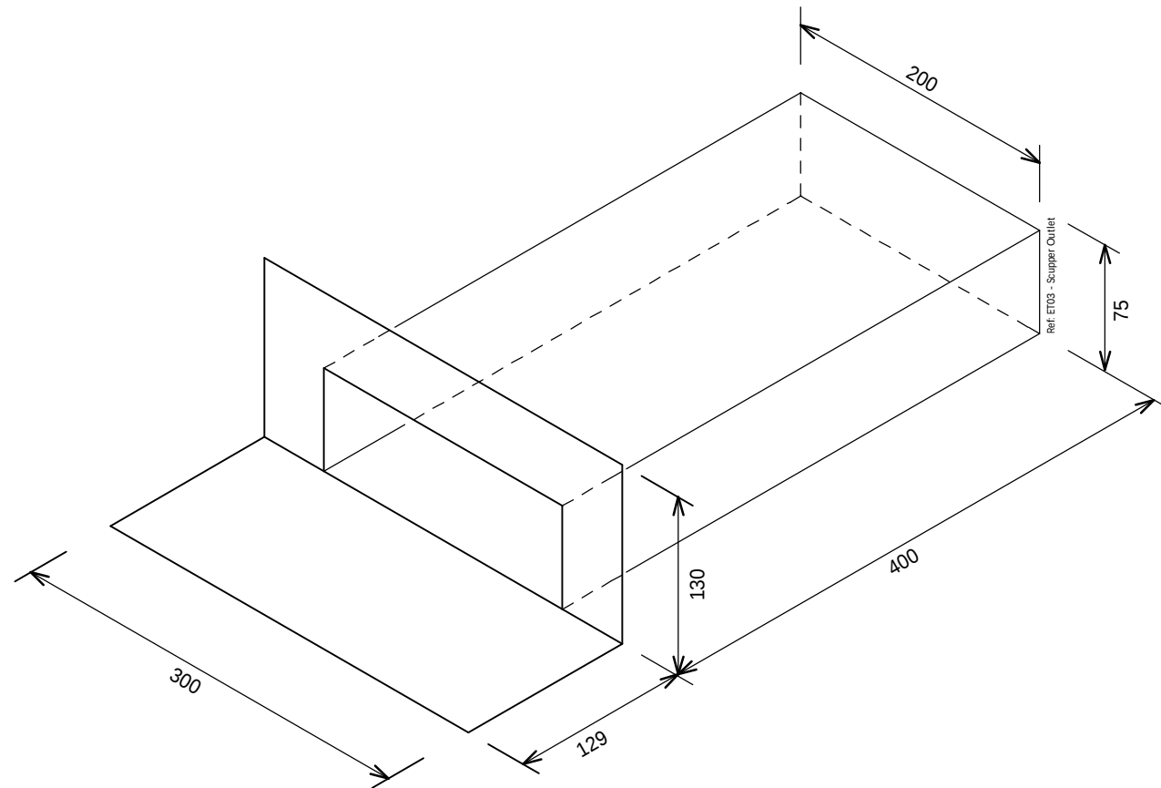
Eterno™ Scupper Outlet 200 x 75mm
