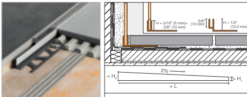
SHOWERPROFILE-S
